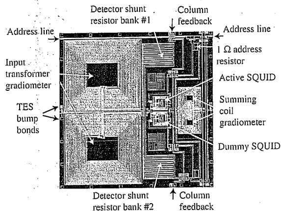
Fig. 3. Labeled photograph of a SCUBA-2 MUX pixel.
