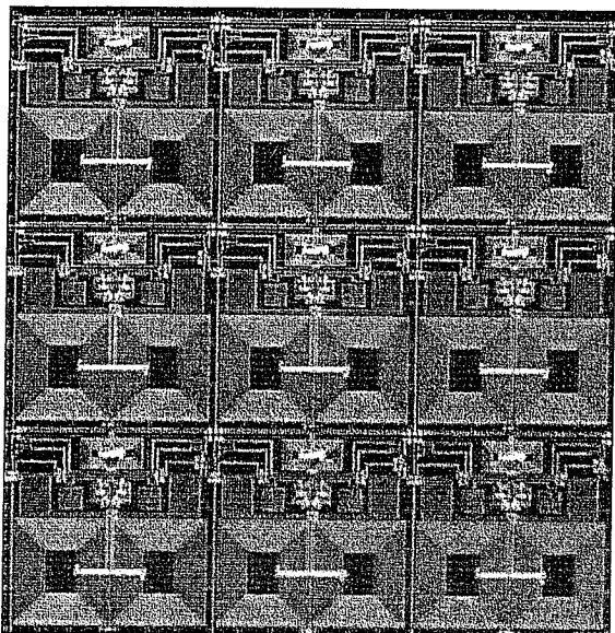
Fig. 4. Photograph of a 3 \times 3 array of MUX pixels. Each pixel is 1.135 mm square.
