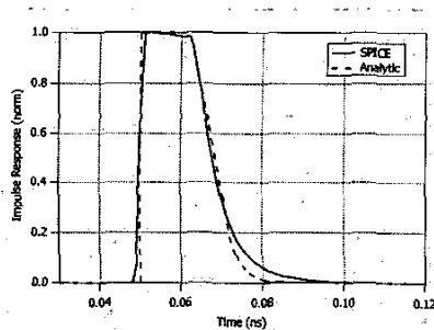
Fig. 5: Impulse response from a SPICE simulation [4] that utilizes an ideal trapezoidal strobe source (solid) and from the analytic model of [9] (dashed). The values of the circuit elements used in the two simulations were similar.
