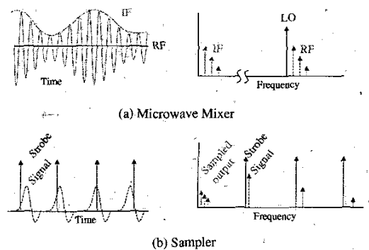
Fig. 6: Microwave-mixer/sampling-oscilloscope analogy.
