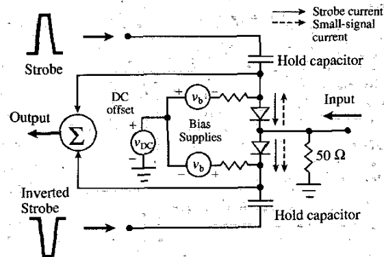
Fig. 1. Simplified electrical model of a sampling circuit.
