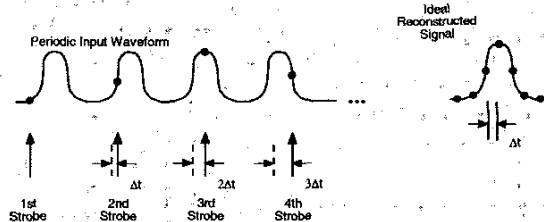
Fig. 2. Ideal sequential sampling and reconstruction.
