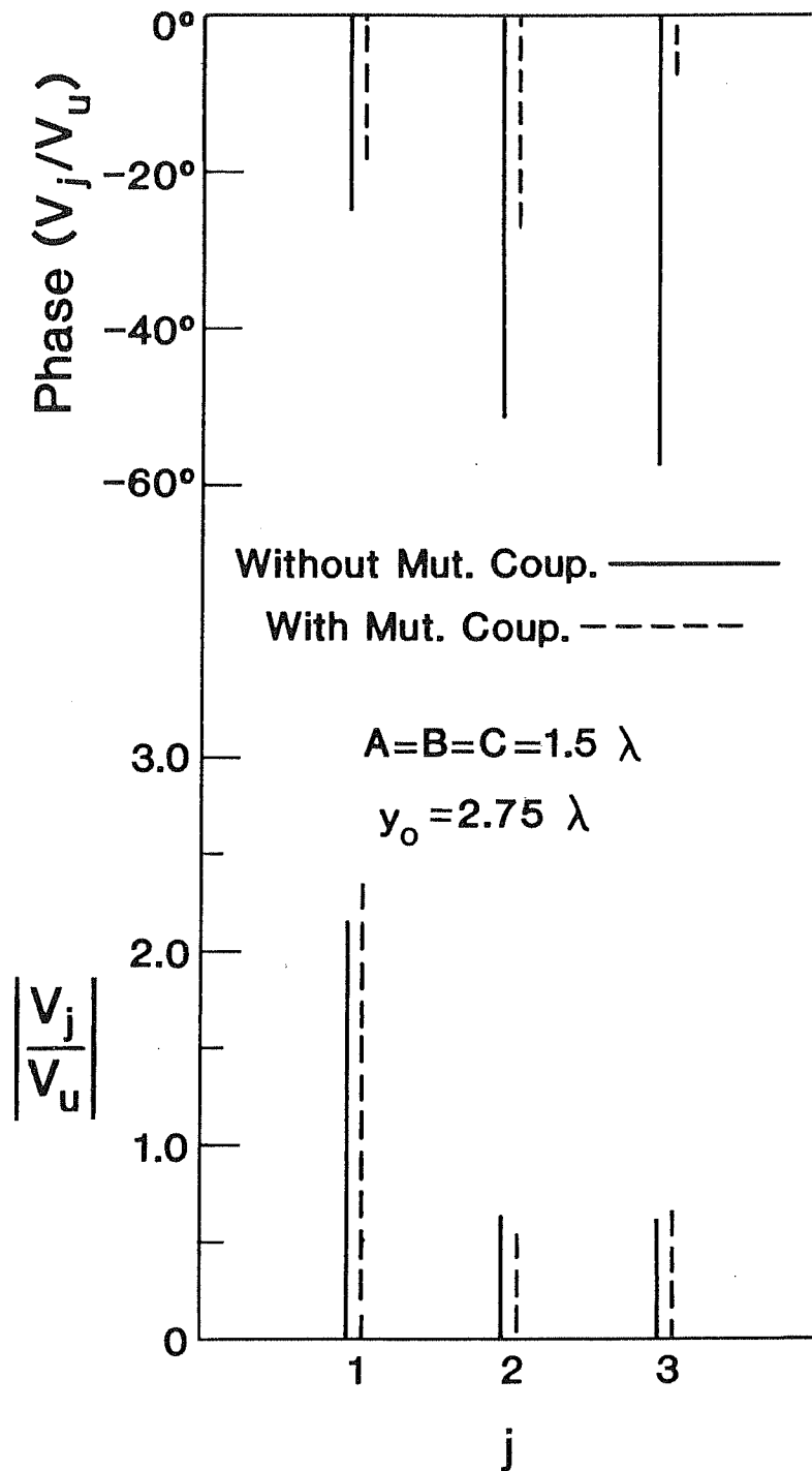
Figure 20. Magnitude and phase of the voltages with and without mutual coupling. These voltages correspond to the currents in figure 13.
