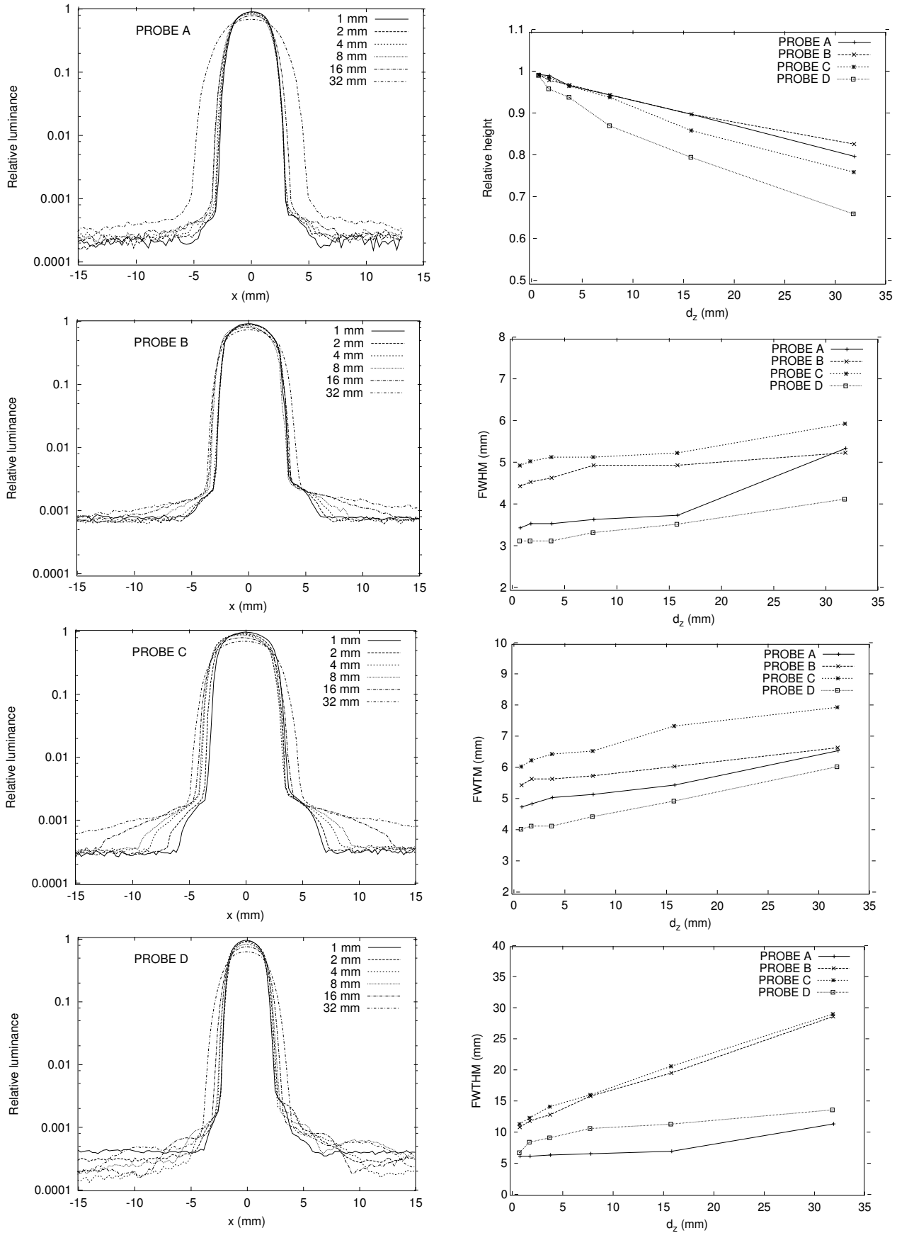
Fig. 3. Luminance scans of a 0.1 mm slit for six d_z for the four probes studied in this work (A-D). Fig. 4. From top to bottom, comparison of scan heights, full-width-at-half-maximum, full-width-at-tenth-maximum, and full-width-at-thousandth-maximum.
