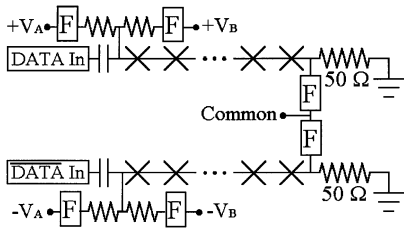
Fig. 4. Diagram of the superconducting integrated circuit for the quantized voltage noise source. Josephson junctions are indicated by Xs and low-pass filters by Fs. The two output voltages V_A and V_B across both arrays are applied to the differential inputs of the two cross-correlation channels.
