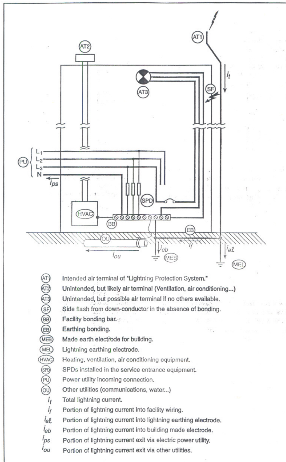
Figure 2 — Example of possible multiple paths for dispersion of the lightning current
