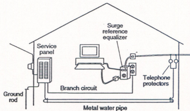
Figure 6 Surge Reference Equalizer for telephone link
