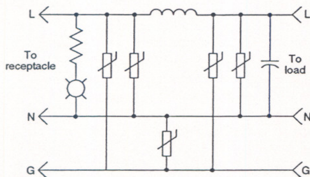
Figure 4 Typical circuit of a power-port, plug-in TVSS
