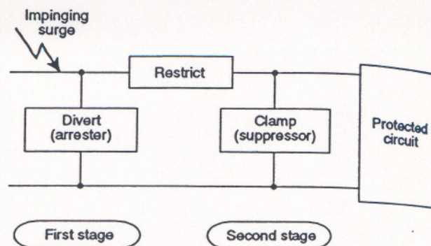
Figure 1 Two-stage surge-protection scheme
