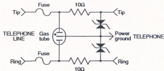
Figure 5 Typical circuit for a telephone port SRE
