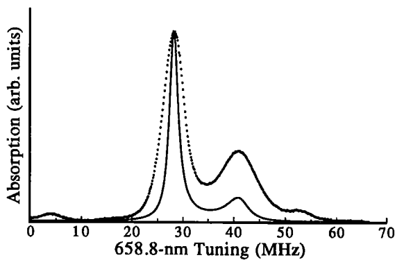
Fig. 3. Theoretical cesium-absorption line shape and experimental data points for 9-MHz detuning of the trapping laser and a Rabi frequency of 11 MHz. The experimental data show sidebands at 4 and 54 MHz that result from 25-MHz modulation of the probe laser. These sidebands are used for determining the frequency scale.
