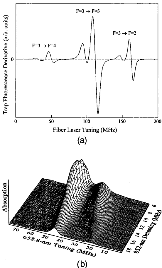
Fig. 2. (a) Rubidium line shape showing the derivative of the 780-nm fluorescence signal as the 1.529- \mu\text{m} fiber laser is scanned through the 5P_{3/2}, F = 3 \rightarrow 4D_{5/2}, F = 4, 3, and 2 transitions. The detuning was -11 \pm 1 MHz, and the Rabi frequency was 8.5 \pm 0.5 MHz. The fiber-laser intensity was 0.7 \pm 0.2 mW/cm 2 . (b) Cesium absorption at 658.8 nm as a function of the probe laser frequency for various trap laser detunings. We improved the signal-to-noise ratio by averaging 200 scans at each detuning. The large peaks on successive lines were aligned to display clearly the change in splitting.
