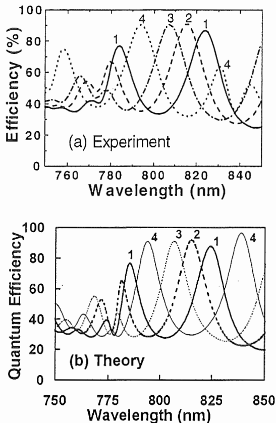
Figure 1: (a) Experimental and (b) theoretical photoresponse of the p-i-n RCE photodiode.
