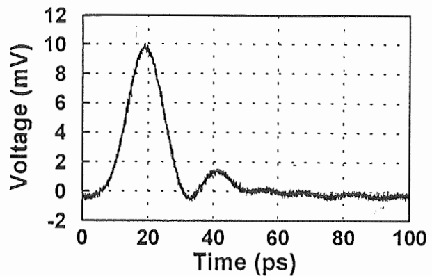
Figure 2: Pulse response of the sample
