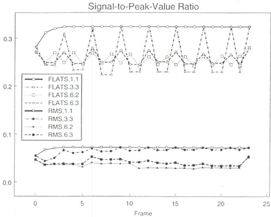
Figure 4: The computed FLATS and RMS frame impairment metrics in units of signal-to-peak-value ratio, as a function of frame number. The upper graphs show the frame-by-frame FLATS metric, F_n , and the lower graphs the RMS metric, R_n . The mosquito noise metrics are based on the average variation in F_n and in R_n .
