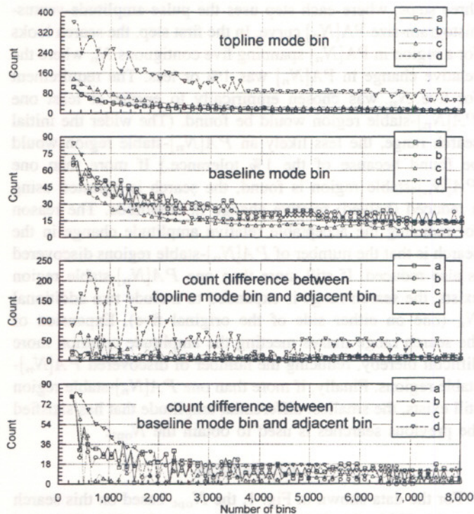
Fig. 7. Various histogram artifacts as a function of the number of histogram bins. The curves labeled (a)–(d) correspond to the curves found in panels (a)–(d) in Fig. 1.
