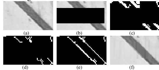
Fig. 7. An example of the proposed error concealment for a portion of the video image "Foreman"; (a) the original image; (b) the image with packet loss; (c) the edge map after Sobel operator; (d) the edge map after thinning; (e) the edge map after Hough transform; (f) the concealed image after region-based interpolation.
