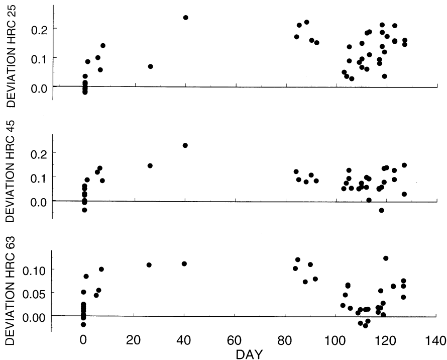
Fig. 6. Long-term variation shown for each day by the difference between a cross-hexagon pair and the center.
