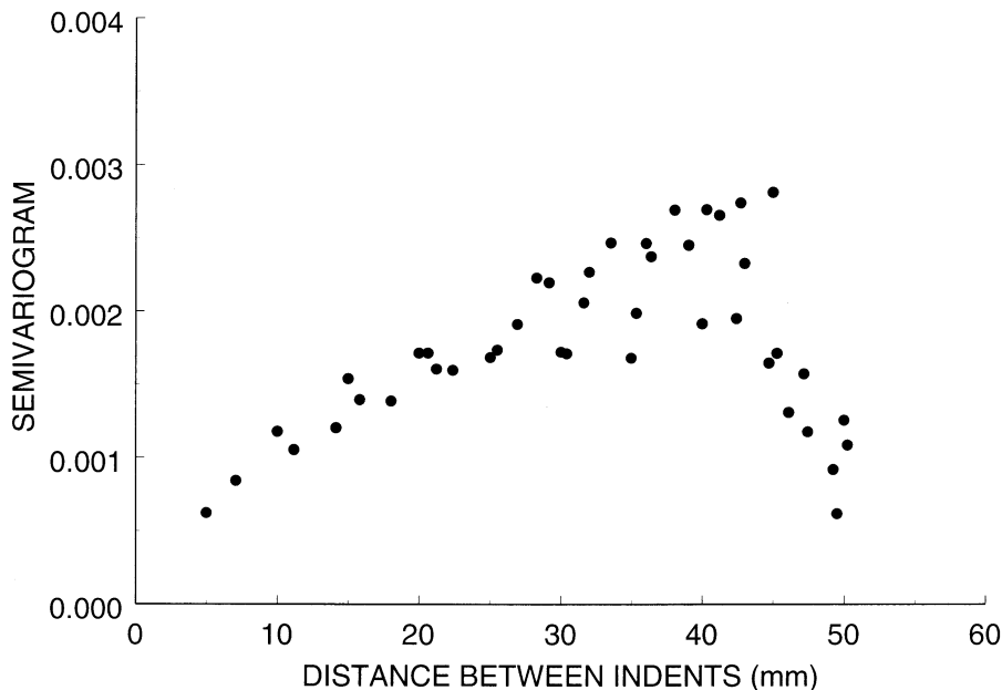
Fig. 8. Empirical semivariogram for block 95N63001 (one half the mean square of differences).
