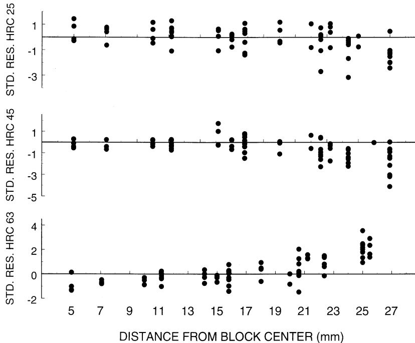
Fig. 11. Measured value minus predicted value divided by standard deviation of the predicted value for a block of each hardness level.
