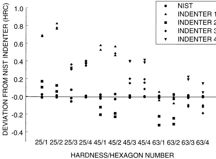
Fig. 7. Measurements with five indenters given as deviations from the averages of measurements with the NIST indenter.
