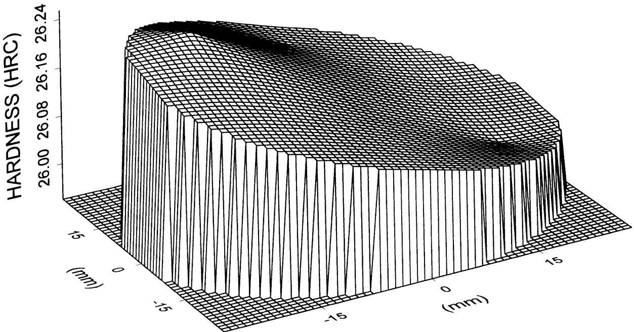
Fig. 10. Hardness values of unmeasured locations on a NIST SRM block predicted from the seven measurements NIST made.
