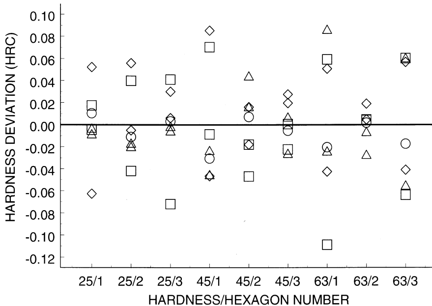
Fig. 5. Repeatability data with different symbols for the center point (circle) and each cross-hexagon pair (triangle, square, or diamond).
