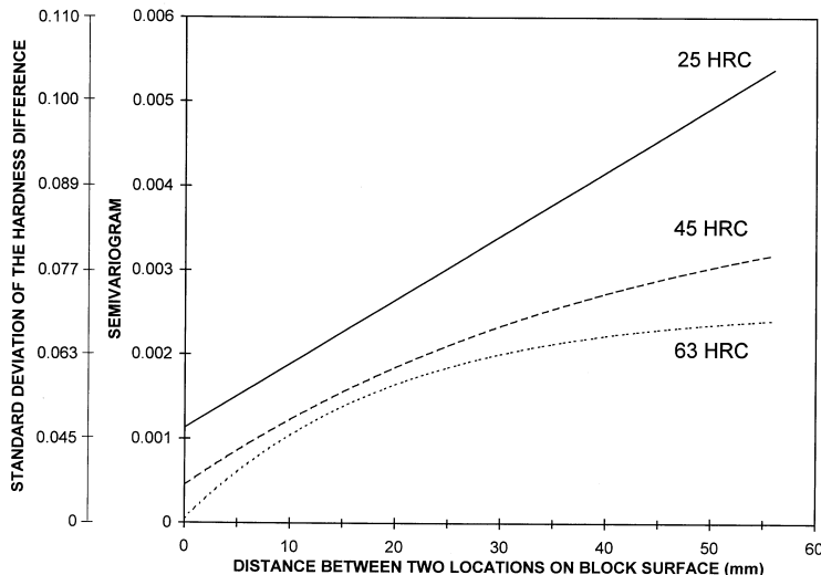
Fig. 9. Semivariogram functions applicable to the first issue of the NIST SRMs.
