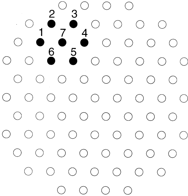
Fig. 4. A 6 mm equilateral triangular grid for a block with a hexagonal measurement pattern highlighted and numbered.
