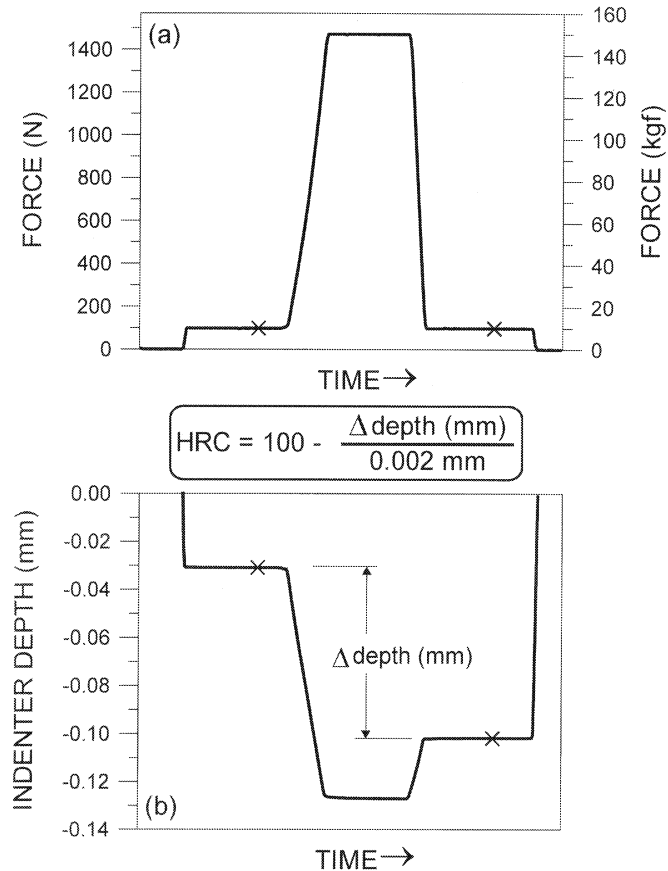
Fig. 1. Rockwell C scale hardness test illustrated with change of force with time (a) and resulting indentation depth (b). Indenter depth measurements used in calculation of hardness value are indicated by × symbol.
