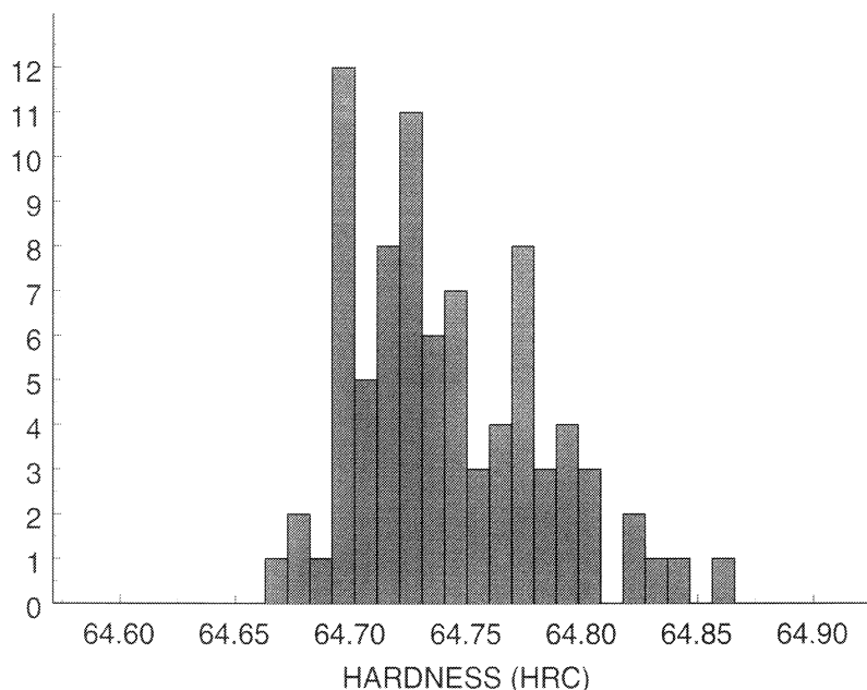
Fig. 2. Histogram of measurements taken on block 95N63001.
