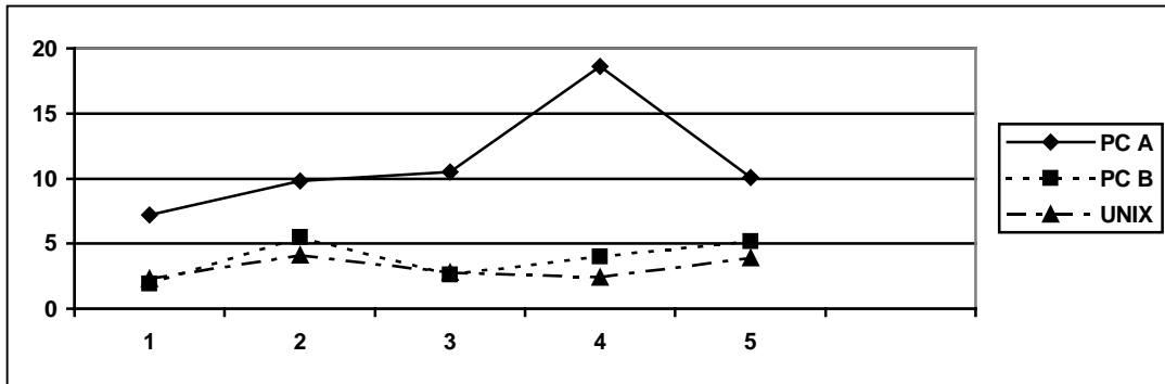
Figure 6. OCR Error Rate on Bad Quality Images
