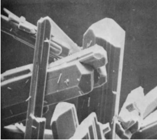
Figure 1: A scanning electron micrograph (900X) [Clifton, 1973] of precipitated gypsum crystals ( CaSO_4 \cdot 2H_2O ).
