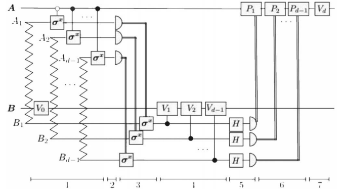
FIG. 8. A nonlocal two-qudit gate U = W^\dagger that realizes the state synthesis U|0\rangle_{A,B} = |\psi\rangle_{A,B} on qudits A and B using d-1 ancillary qubit pairs (indicated by sawtooth lines) each prepared in the state |\phi^+\rangle_{A_j,B_j} = 1/\sqrt{2}(|00\rangle + |11\rangle)_{A_j,B_j} . Each qubit A_j(B_j) in the entangled resource can constitute a new particle or a distinct degree of freedom of qudit A(B) . Controlled-NOT gates between A and A_j are conditioned on the basis state |j\rangle_A , as indicated by the shading of the control bubble. Double lines denote classical controlled operations dependent on qubit measurement outcomes, H = e^{i\pi(\sigma^x + \sigma^z)/2\sqrt{2}} , and P_j = e^{i\pi|j\rangle\langle j|} . The sequence of steps that can be implemented in parallel is indicated at the bottom.
