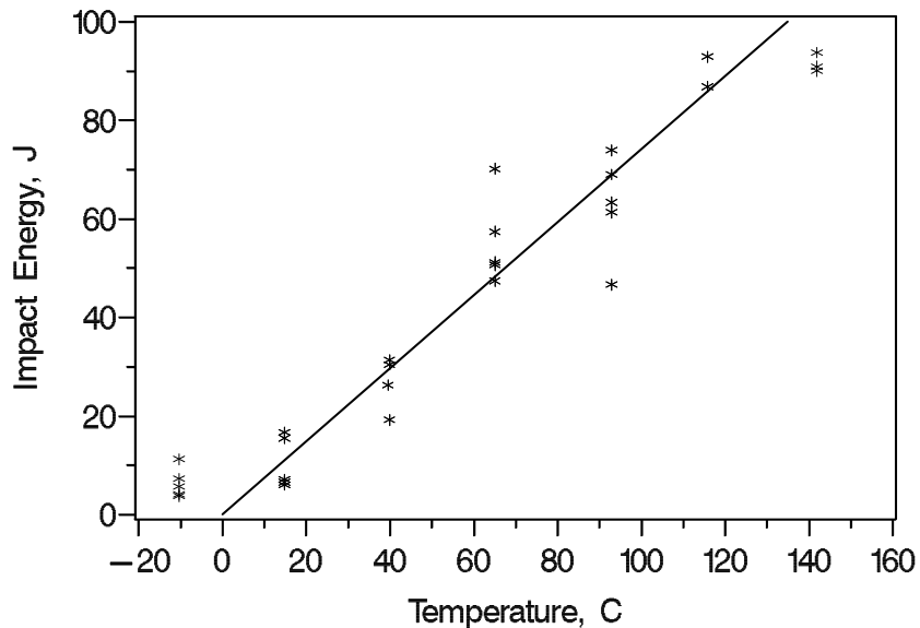
Figure 3. Temperature data for the test material. The straight line in the plot represents a regression fit to the data in the transition region only. We ignore data on the “shelves” at -10^{\circ}\text{C} and 141^{\circ}\text{C} .
