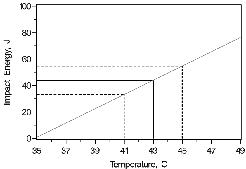
Figure 2. Mapping of temperature error into energy error in the temperature transition region.
