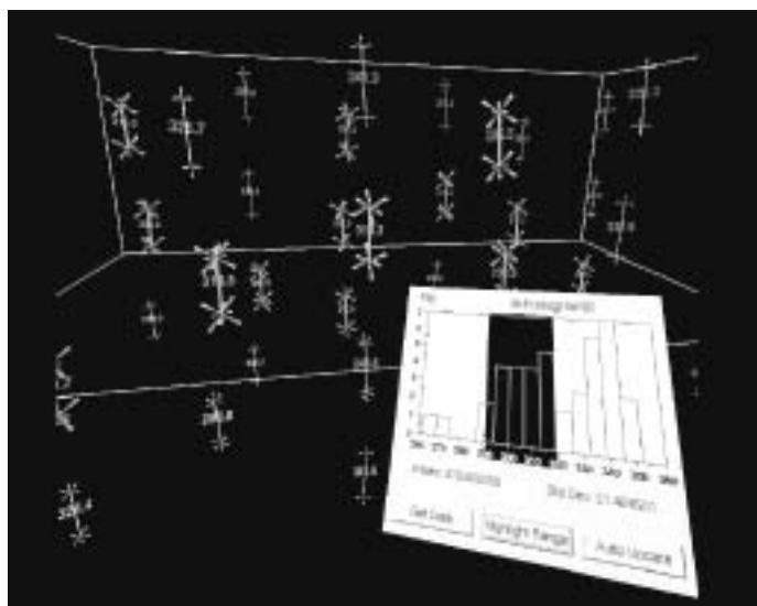
Figure 4. Selected histogram bins are highlighted in visualization showing distribution of strut diameters in the range of 200 to 320 \mu\text{m} . The struts have been removed from the scene in order to make the measurements more visible.
