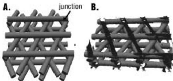
Figure 2. As-designed scaffold, synthetically constructed based on the design specifications (A.), 3D reconstruction of the scaffold made by SFF (B.).
