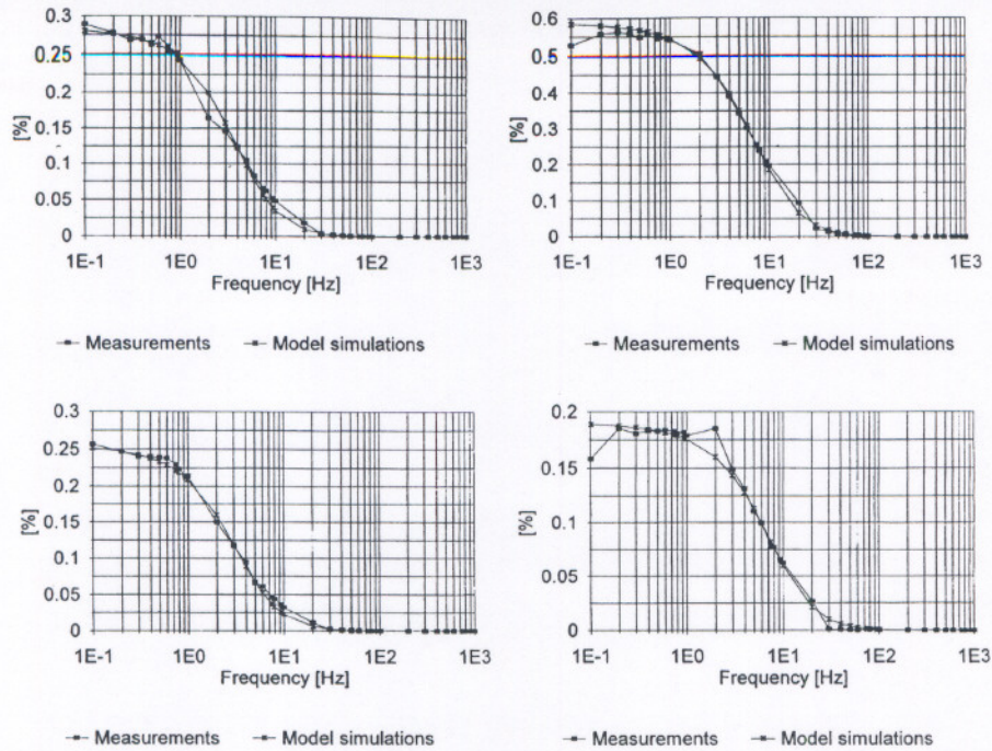
Fig. 2. Model simulations and measurements of ac-dc differences versus frequency for TVC's A, B, C, and D.
