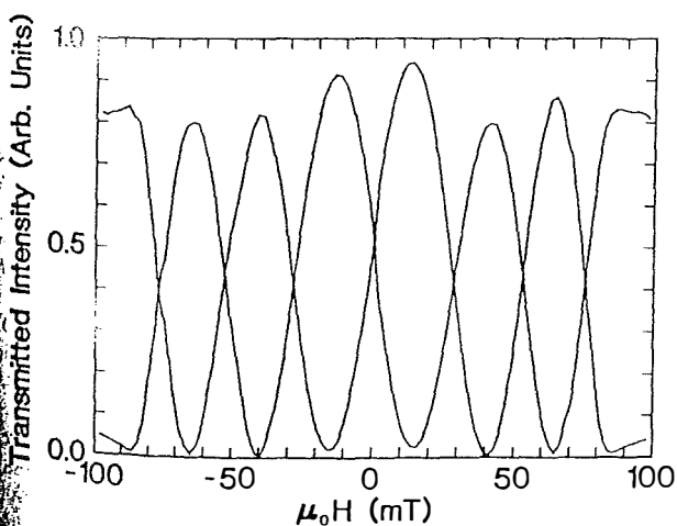
Fig. 3. Measured magneto-optic responses for Film 2.
