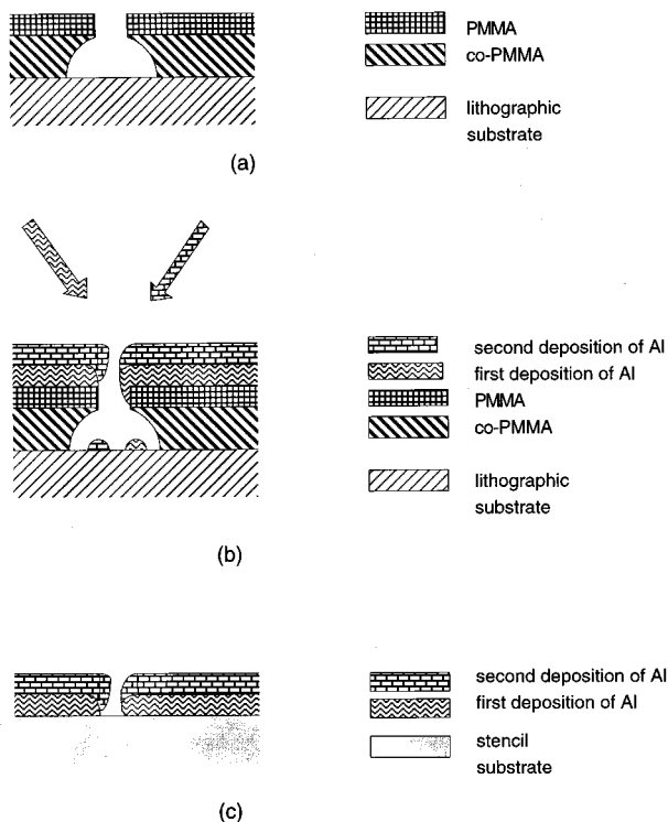
FIG. 1. Schematic of the procedure: (a) after lithographic exposure and development of the bilayer resist; (b) after deposition of metal at two different angles, yielding asymmetric film profiles; (c) after liftoff and recapture of the stencil onto a different (possibly with open holes) substrate. Note that the dual-angle deposition yields the potential for a stencil opening substantially smaller than the lithographically produced one.
