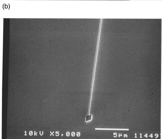
FIG. 2. SEM micrographs of a 100-nm-thick stencil captured onto a Si wafer, at an oblique tilt of about 50^\circ , and three different magnifications. Note the well-formed nature of the square hole and trench; the firm edges, and that the stencil has flattened against the solid substrate. Note also the absence of any pinholes or other imperfections.
