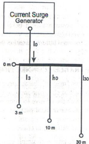
Figure 2 — Test circuit for cascade coordination
