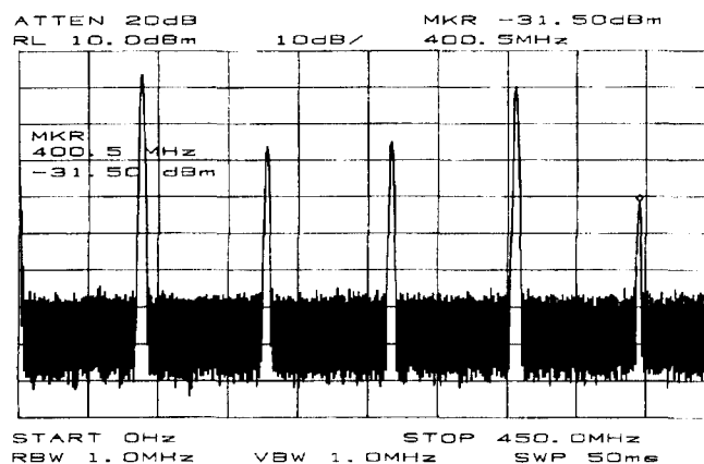
Fig. 7 Regenerative divide-by-three operation
