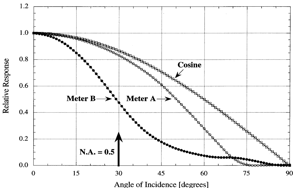
Fig. 6. Angular response of two UV meters.
