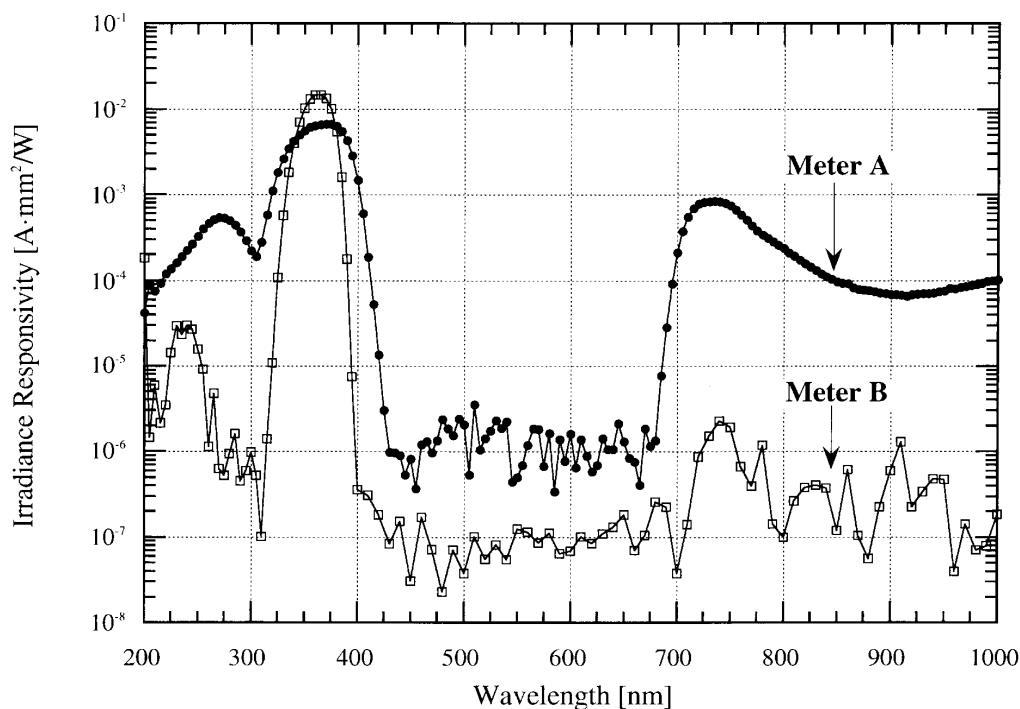
Fig. 3. Spectral responsivity of two UV irradiance meters. Uncertainties for these data are given in Ref. [4].
