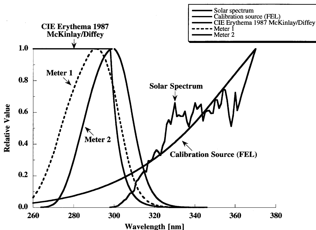
Fig. 8. Spectral responsivities of two UV radiometers plotted with the CIE 1987 erythema function and spectral power distribution of an FEL lamp and the solar spectrum. (Fig. 3 in Ref. [6].)
