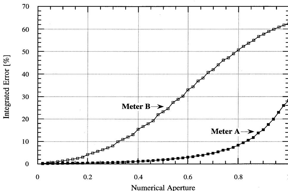
Fig. 7. Integrated error due to cosine response.
