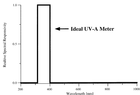
Fig. 2. Spectral responsivity of an ideal UV-A meter.
