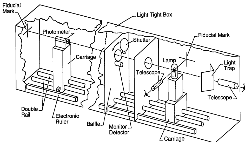
Fig. 6. New NIST photometry bench.
