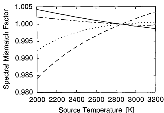
Fig. 5. Effect on photometer calibration when sources at different temperatures are viewed. The required correction is reported as F(\text{Temp})/F(2856 \text{ K}) . Representative packages: Photometer 2, dashed curve; photometer 3, dotted curve; photometer 5, solid curve; photometer 8, dashed-dot curve.
