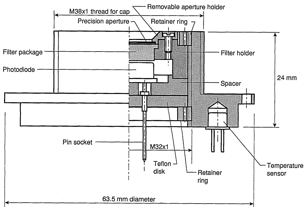
Fig. 2. Photometer design. A filter modifies the spectral response of a silicon photodiode to replicate as closely as possible the 1924 CIE Spectral Luminous Efficiency Function for Photopic Vision.
