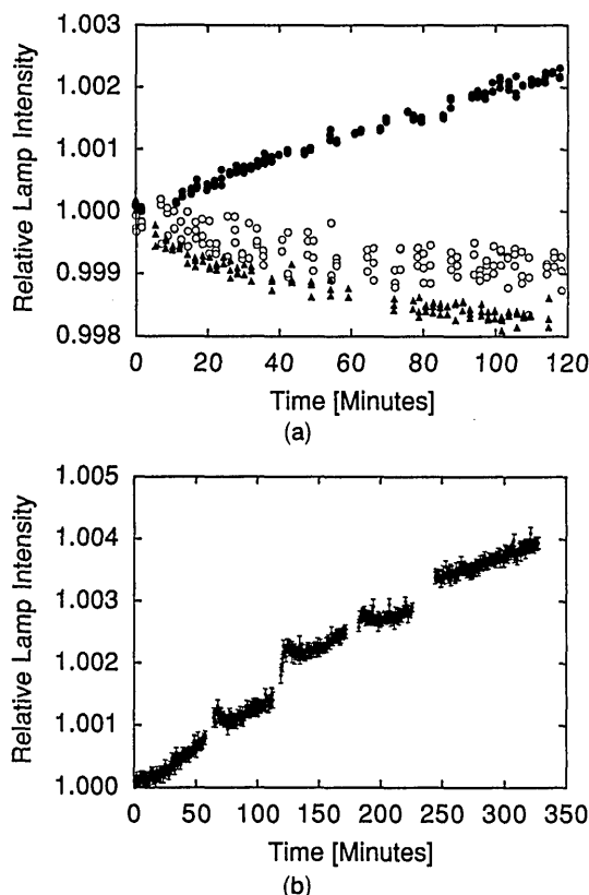
Fig. 7. Drift and noise in the output of representative standard lamps: (a) During one lighting of an Osram Wi 41/G lamp, ●; a FEL, ○; and an inside-frosted T-20 lamp, ▲. (b) During five consecutive lightings of the Osram lamp.
