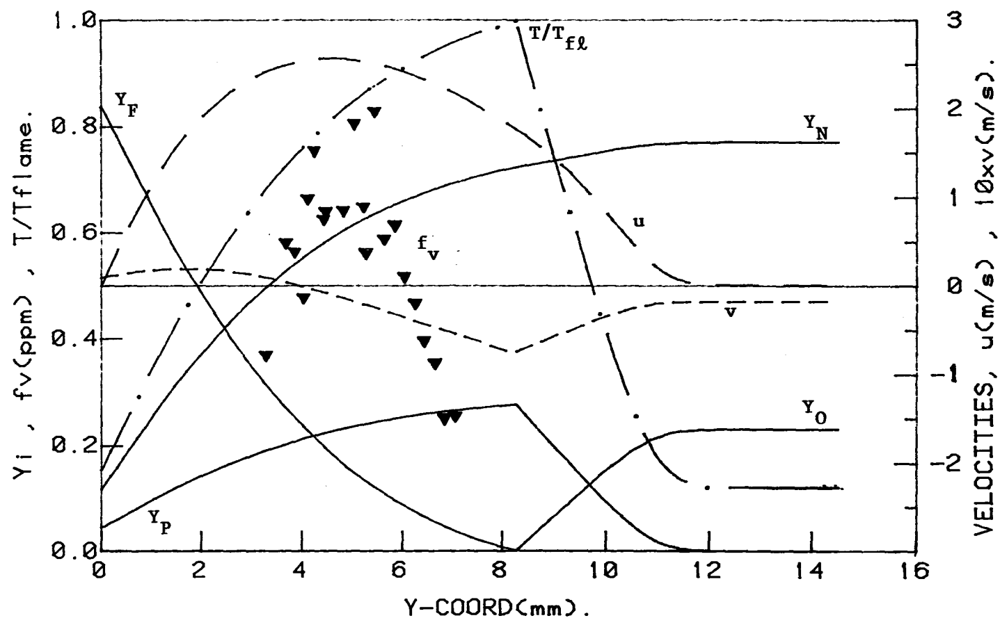
Fig. 1b. Velocity, temperature, species, and soot profiles as in Fig. 1a, except here the distance from the leading edge is 100 mm to show the evolution of the soot volume fraction profile. The soot exists primarily in the region between the converging streamline ( v = 0 ) and the flame ( Y_F = Y_O = 0 ).
