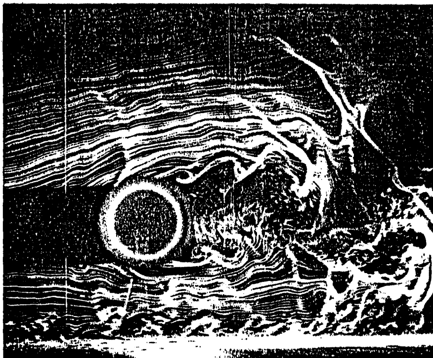
Figure 1. Smoke wire flow visualization of flow around cylinder located 1.1 diameters above the floor. Re_D = 5200
