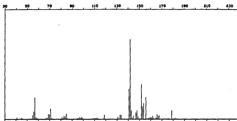
Figure 4. Factor spectrum of gasoline.
