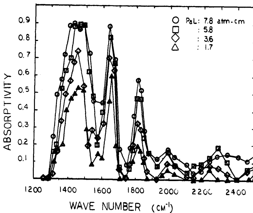
Fig. 1: Spectral absorption of Propylene near the \nu_7 ( 1473 \text{ cm}^{-1} ) and \nu_6 ( 1651 \text{ cm}^{-1} ) fundamental bands and the 2\nu_{19} ( 1825 \text{ cm}^{-1} ) first overtone band.
