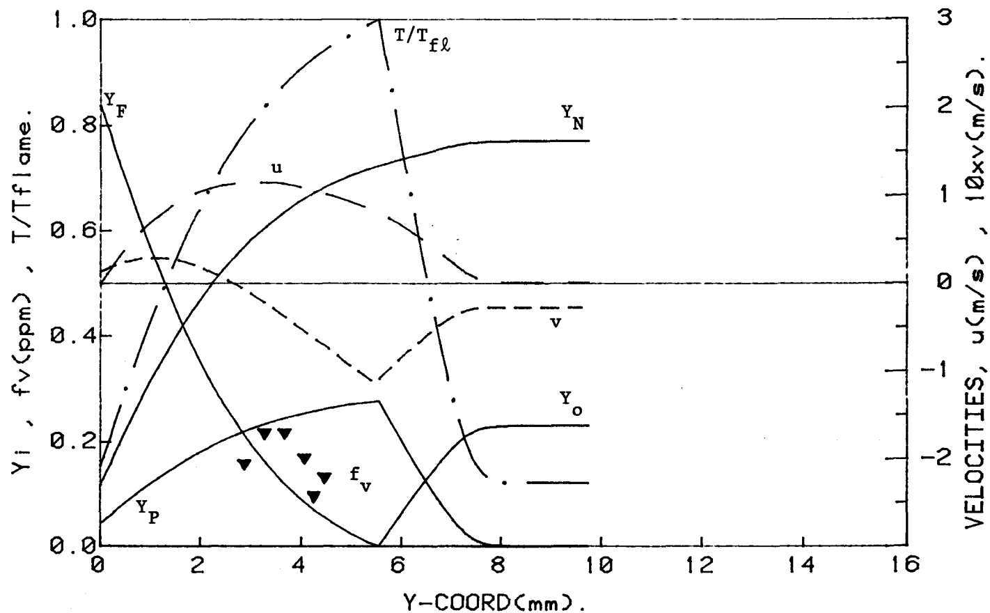
Fig. 1a. Velocity, temperature, species, and soot profiles in an n-heptane/air free flow boundary layer flame at 20 mm from the leading edge. Radiation effects are included. The calculated non-adiabatic flame temperature is T_{flame} = 2424 K. The pertinent dimensionless parameters are B = 5.6 , D_c = 29.0 and r = 0.078 .
