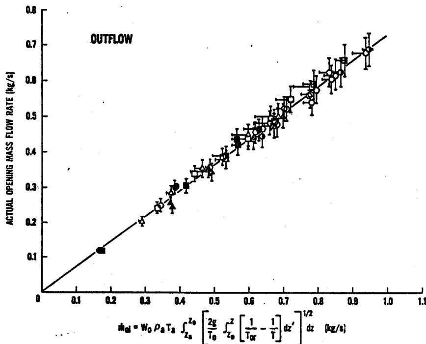
Figure 3. Mass flow rate derived from temperature data
