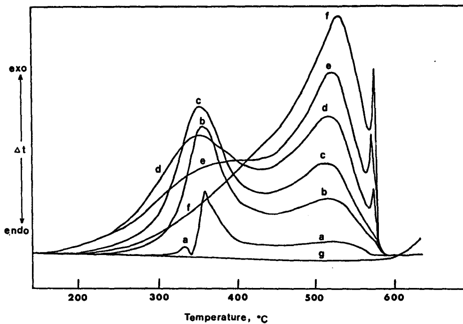
Figure 2. Differential scanning calorimetric curves of cellulosic chars measured in a stream of air. a = cellulose; b-f = cellulosic chars prepared by 5 min heating in N_2 at 340(b), 350(c), 400(d), 500(e), and 600°C(f), respectively; g - graphite.
