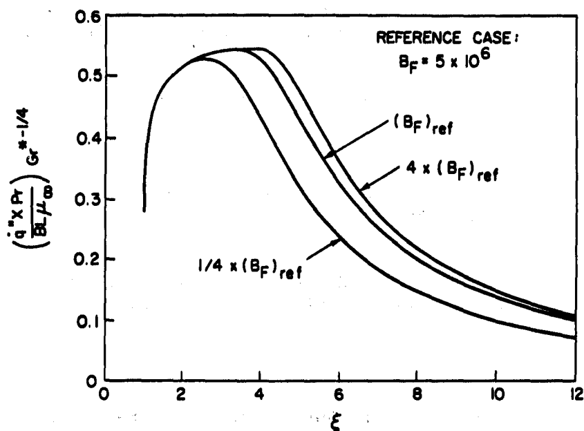
Fig. 1 Nondimensional surface heat transfer rates vs. nondimensional distance \xi , the effect of non-dimensional fuel frequency factor variation. The plume starts at \xi=1 , pyrolysis region is from \xi=0 to \xi=1 .
