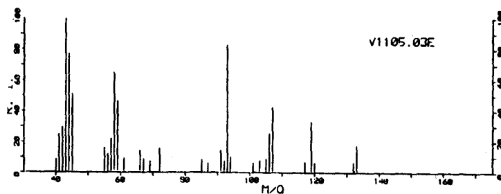
Figure 2. Py-MS spectrum of polyurethane
