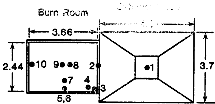
PLAN VIEW (ceiling of room removed)
