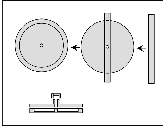
Figure 6.4 Assembly of the Micromolded Pieces
