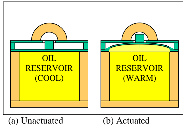
Figure 2.5 Final Assembly of Refrigerant Expansion Device Components
