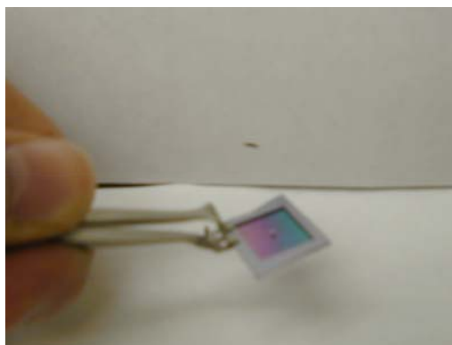
Figure 4.6b Piston/Diaphragm Device
