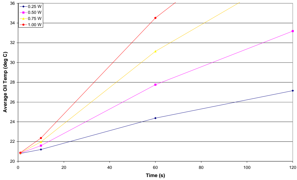
Figure 7.12 Immediate Response of Device to Heat Input
