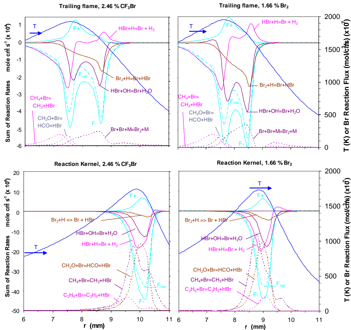
Figure 5 – Detail from Figure 4 of sum of reaction rates for all reactions involving H, O, or OH, with addition of 2.46 % CF 3 Br (left frames) or 1.66 % Br 2 (right frames); top figure: trailing diffusion flame, bottom figure: reaction kernel. For radical consumption, the total is shown for all halogen reactions (F-), as well as the contribution from radical reaction with specific reactions of HBr or Br 2 . In both flames (top and bottom frames), the important reactions reforming HBr and Br 2 are also shown (dotted lines, right scale).
