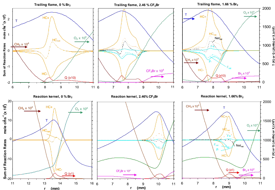
Figure 4 – Sum of reaction rates (left scale) of all reactions involving H, O, or OH, for CH 4 -air cup-burner flame with no agent (left), 2.46 % CF 3 Br (middle) or 1.66 % Br 2 (right). The top frames: trailing diffusion flame; bottom: reaction kernel. Curves are shown for production (+), consumption (-) and the summed (net) effect on radical fluxes, for the halogen (F) and hydrocarbon (HC) reactions. Also shown (using the right scale) are the temperature and heat release, as well as the species volume fraction for O 2 , CH 4 , and CF 3 Br or Br 2 (curve labels in the middle frames are the same as the right frames unless otherwise marked).
