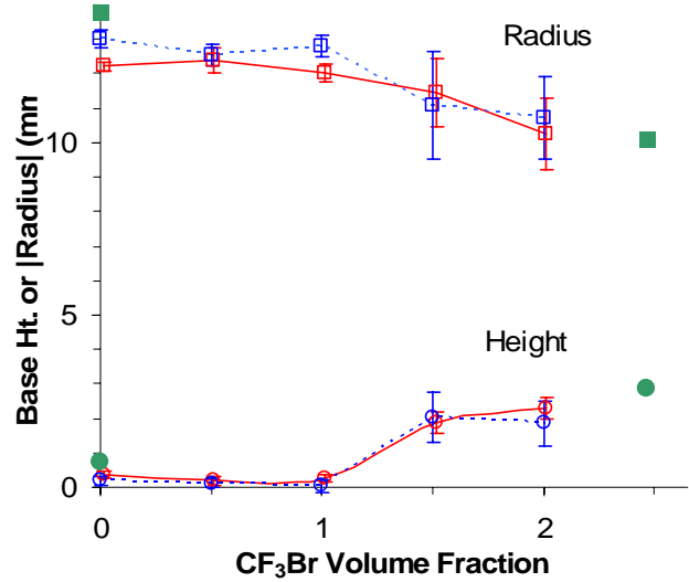
Figure 1 – Measured and calculated flame base radius and height for left (dotted) and right (solid) image of flame base with added \text{CF}_3\text{Br} . The larger solid green points at 0 % and 2.5 % \text{CF}_3\text{Br} are the model prediction.
