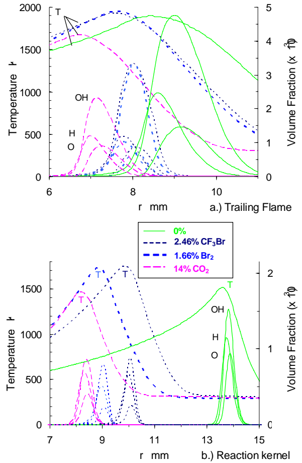
Figure 3 – Flame structures in (a) trailing diffusion flame (top), and (b) reaction kernel (bottom) regions of a cup-burner flame with 0 % and 2.46 % \text{CF}_3\text{Br} , 1.66 % \text{Br}_2 , or 14 % \text{CO}_2 added to the airflow.
