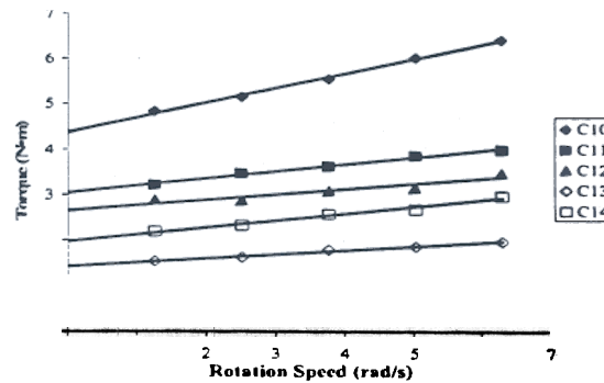
Figure 3. Flow curves obtained with ICAR rheometer
