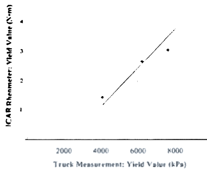
Figure 7. Correlation of yield value between ICAR rheometer and truck
