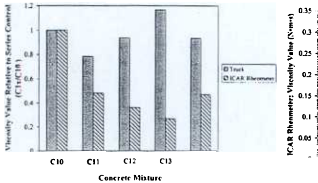
Figure 4. Relative plastic viscosity, recorded by the mixing truck and ICAR rheometer
