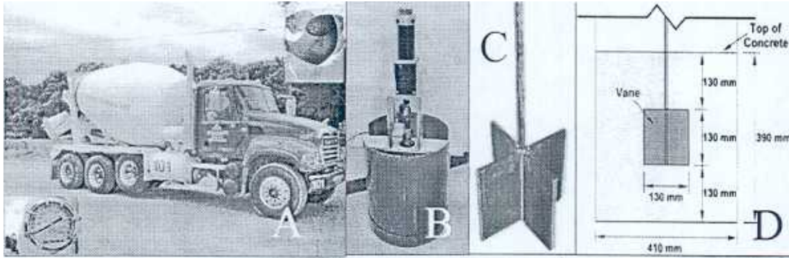
Figure 1. View of the truck (A), the slump indicator (bottom left-a) the interior of the drum (top right-a); the ICAR rheometer prototype (B), vane (C), principal dimensions (D)
