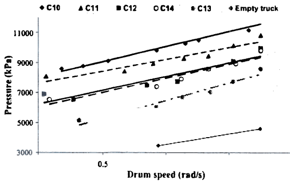
Figure 2. Flow curves obtained with truck mixer
