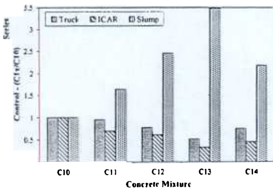
Figure 6. Relative yield or slump values, as recorded by mixing truck, ICAR rheometer, and slump test
